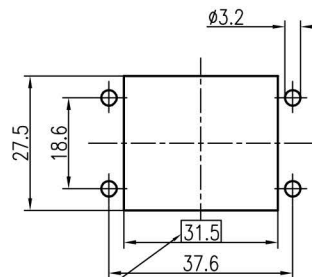
面板开孔图 Panel cut out
